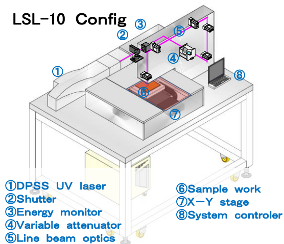
LSL-10 Lab Kit
